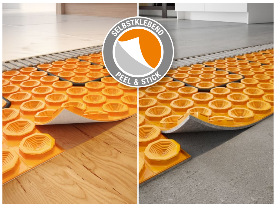
Schlüter®-DITRA-HEAT-PS
